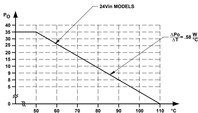
FIGURE 2A. Typical derating curve with free air convection
