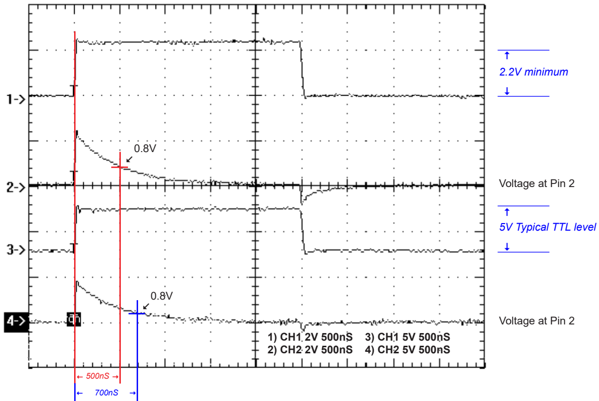
FIGURE 4. Waveforms of sync signal shaping
