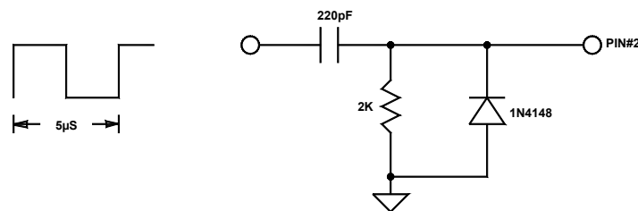
FIGURE 5. Suggested pulse-shaping circuit
