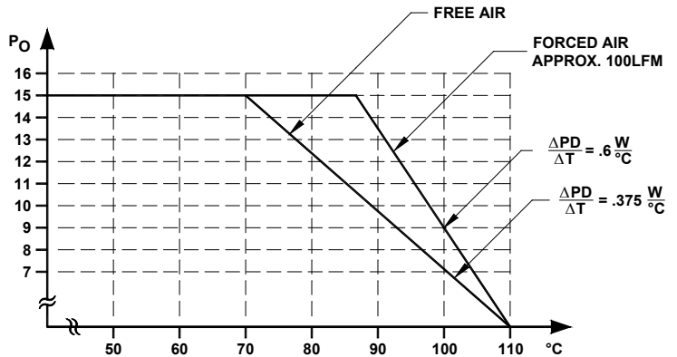
FIGURE 2. Worst case derating of BD30002
