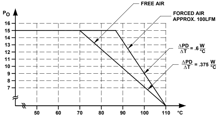
FIGURE 2. Worst case derating of BD30001
