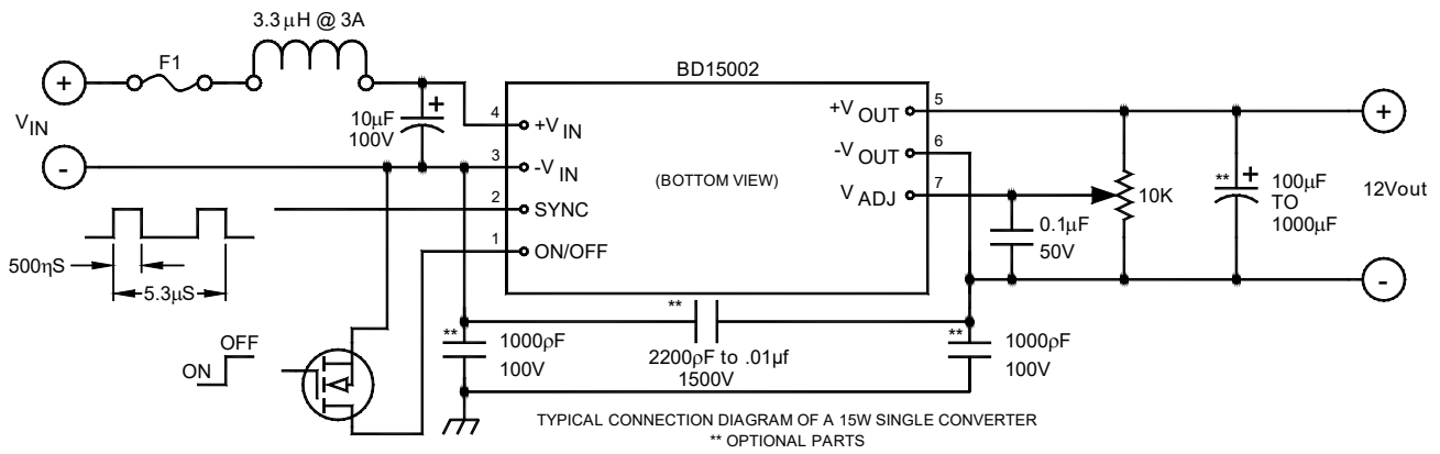
FIGURE 2. Typical connection diagram
