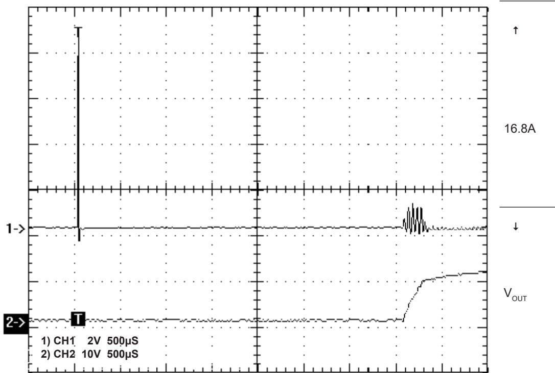
FIGURE 4A. (CH1) Inrush current without hot pluggable circuit ON V_{IN} 48V, Current spike duration 5µS
