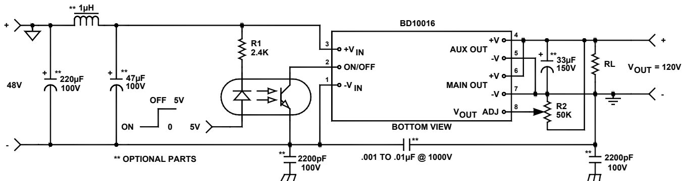
FIGURE 1. Single connection diagram
