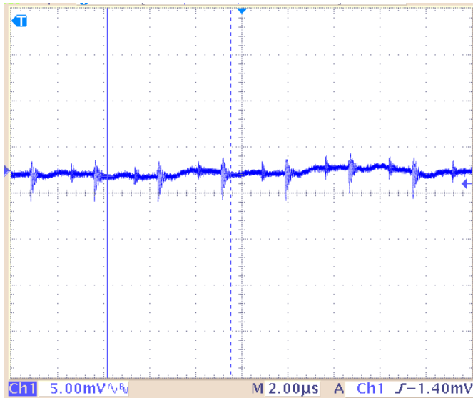
FIGURE 4. Typical output ripple of LN10028, V_{IN}=48V , V_{OUT}=5.5V@1.80A as shown if Figure3.
