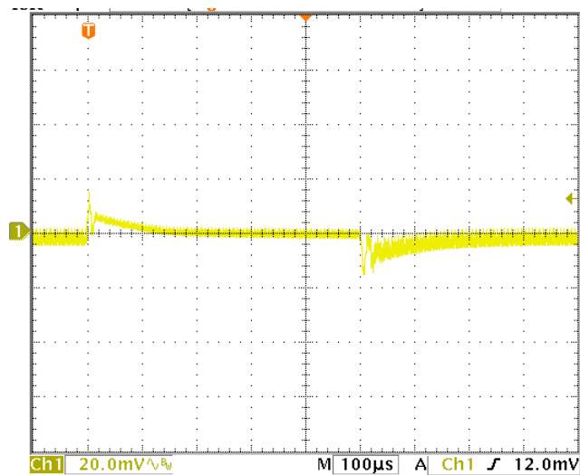
FIGURE 1. Transient response and turn on delay with soft start
