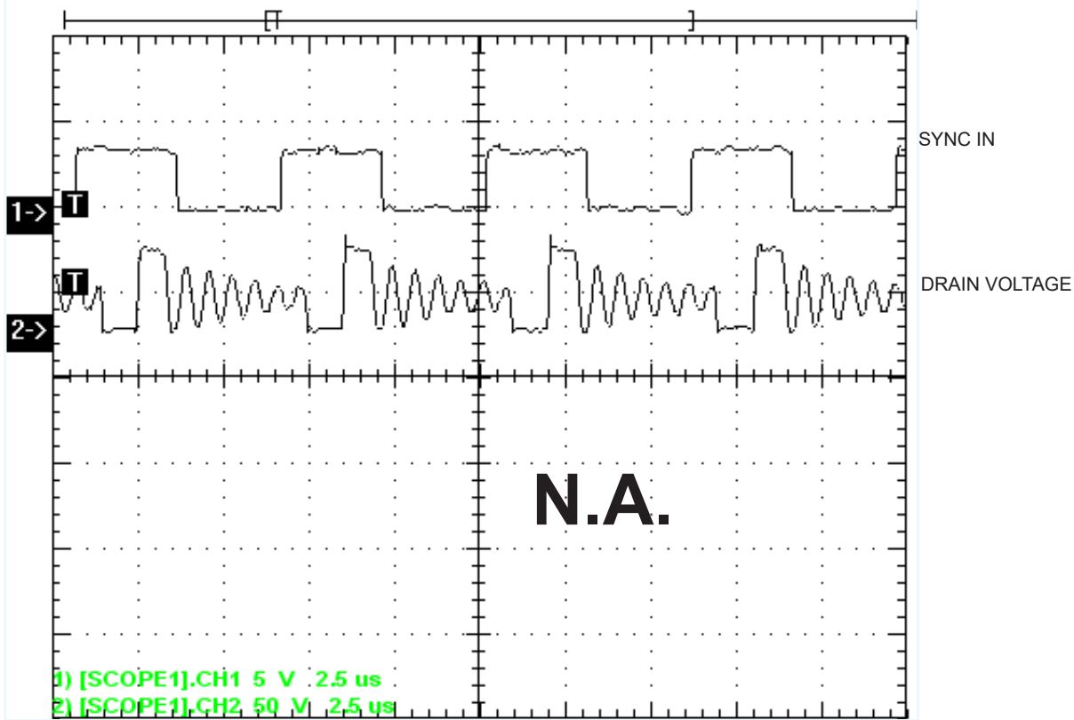
FIGURE 4 . External Synchronization
