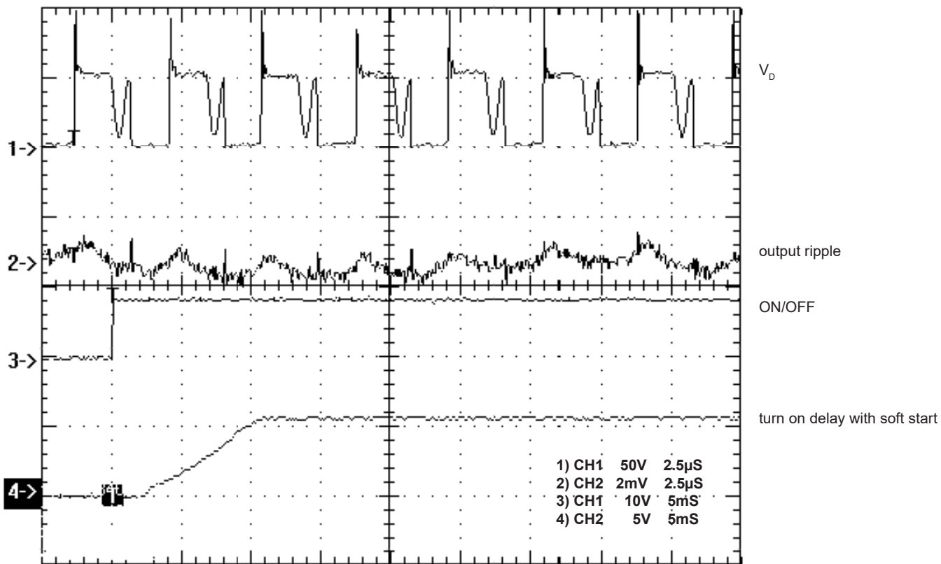
FIGURE 2. Output Ripple and Soft Start of M10001
