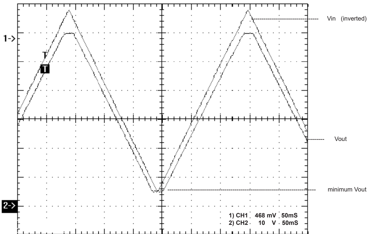
FIGURE 3. V_{out} V V_{in} of M10001
