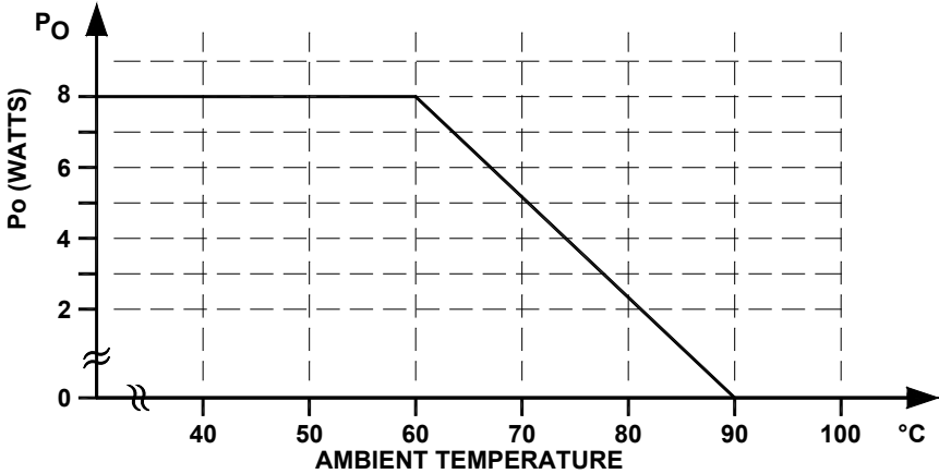
FIGURE 1. Typical derating curve of the M10001
