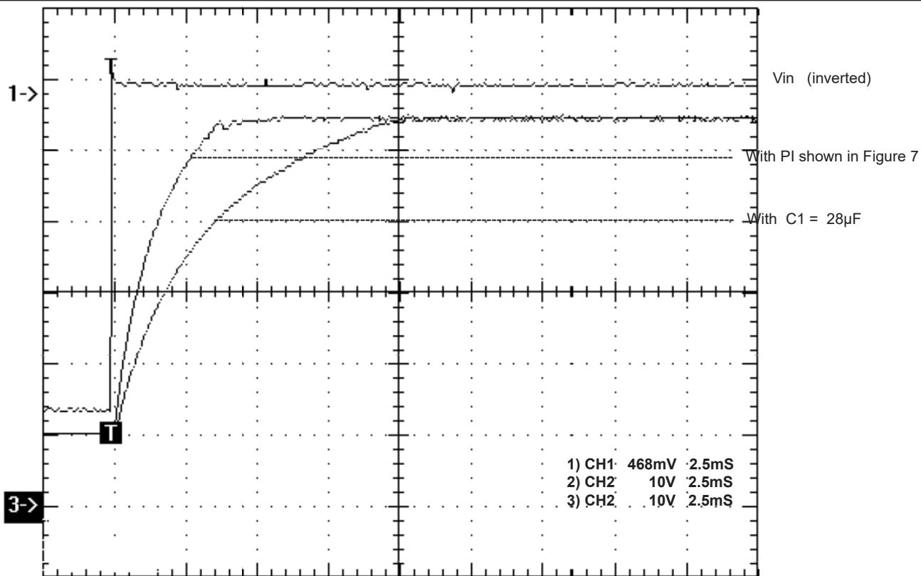
FIGURE 4. Rise time of M10001 with 22 \mu F and without 22 \mu F at C1 (refer to Figure 7)
