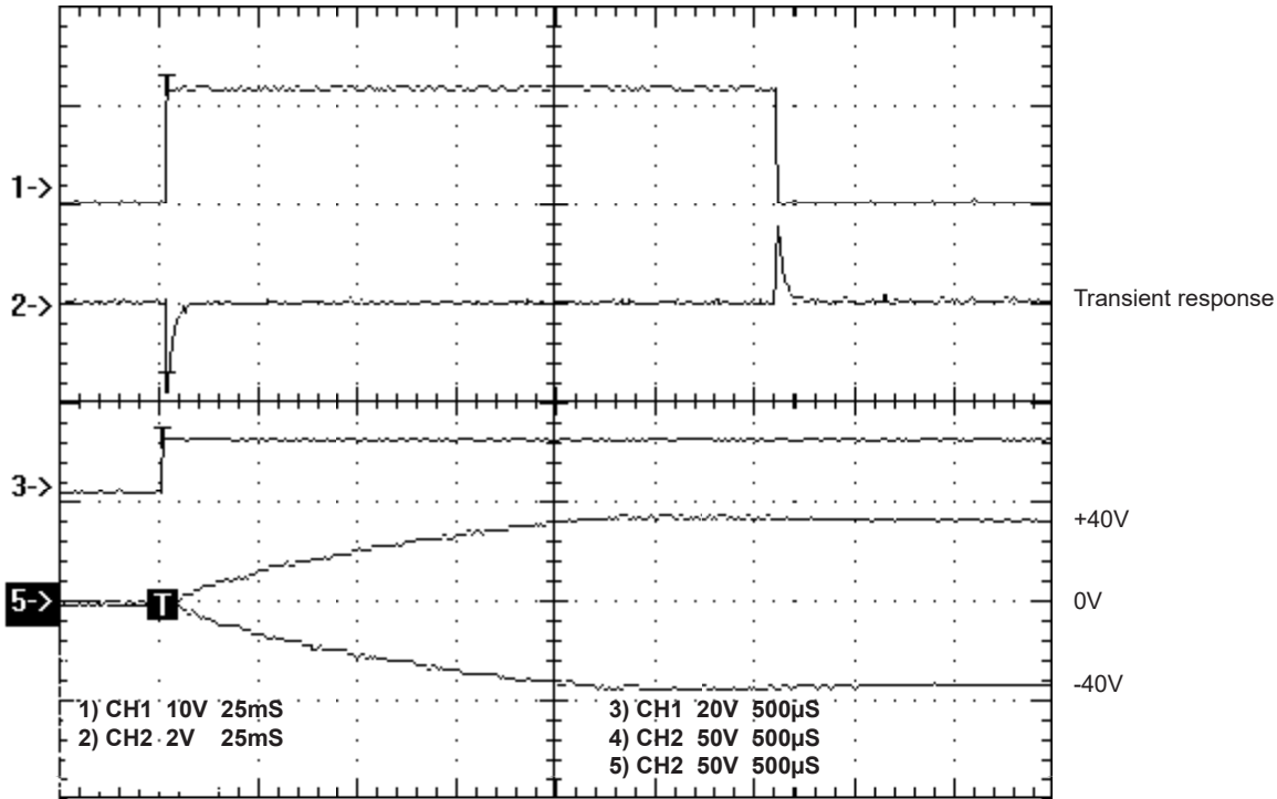
FIGURE 1. Transient response and turn on delay with soft start
