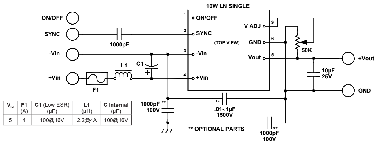
FIGURE 2. Typical connection diagram of Low-Noise 10W Single DC/DC Converter
