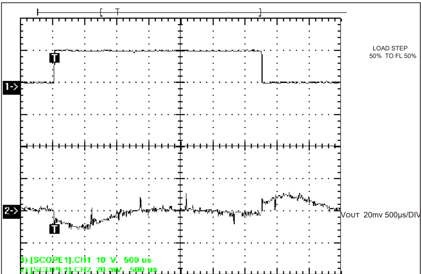
FIGURE 2. TRANSIENT RESPONSE
