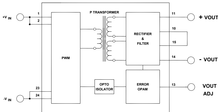
Typical Block Diagram
