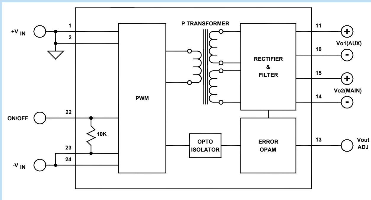
Typical Block Diagram
