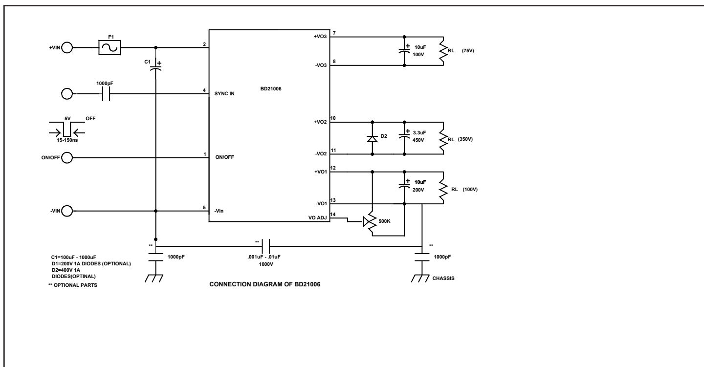
FIGURE 1. Connection diagram
