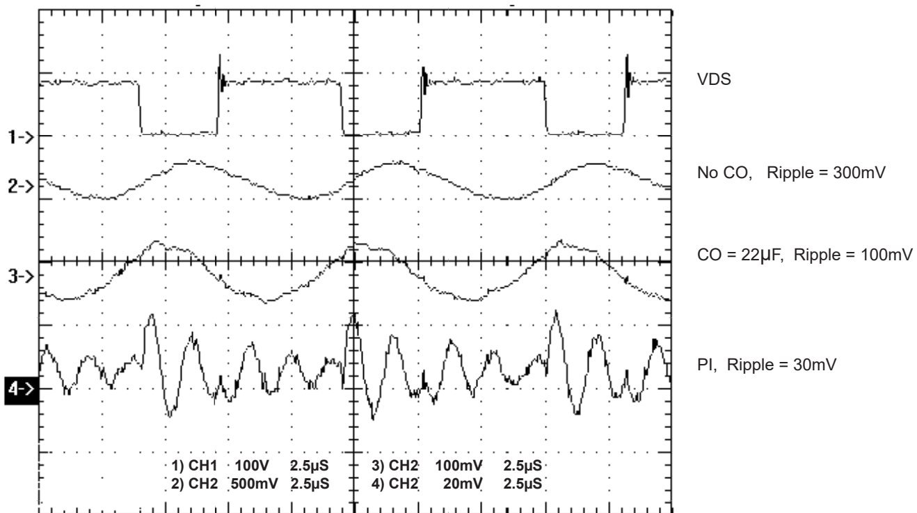
FIGURE 4. Output Ripple
