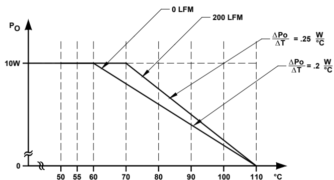
FIGURE 7. Derating of BD10017
