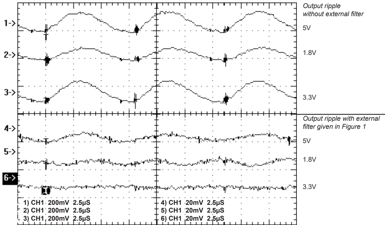
FIGURE 4. Output ripple without and with external filter
