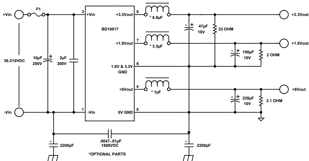
FIGURE 1. Connection diagram
