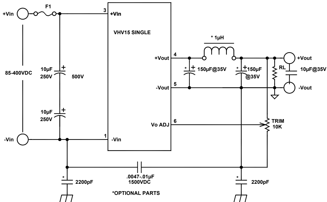
FIGURE 1. Typical Connection diagram for VHV15 SINGLE
