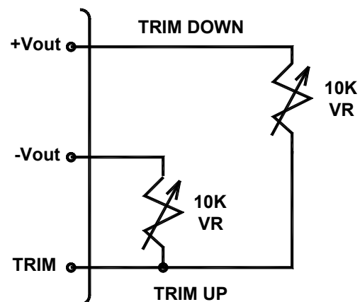
Figure 2. Remote ON/OFF Control & Trim
