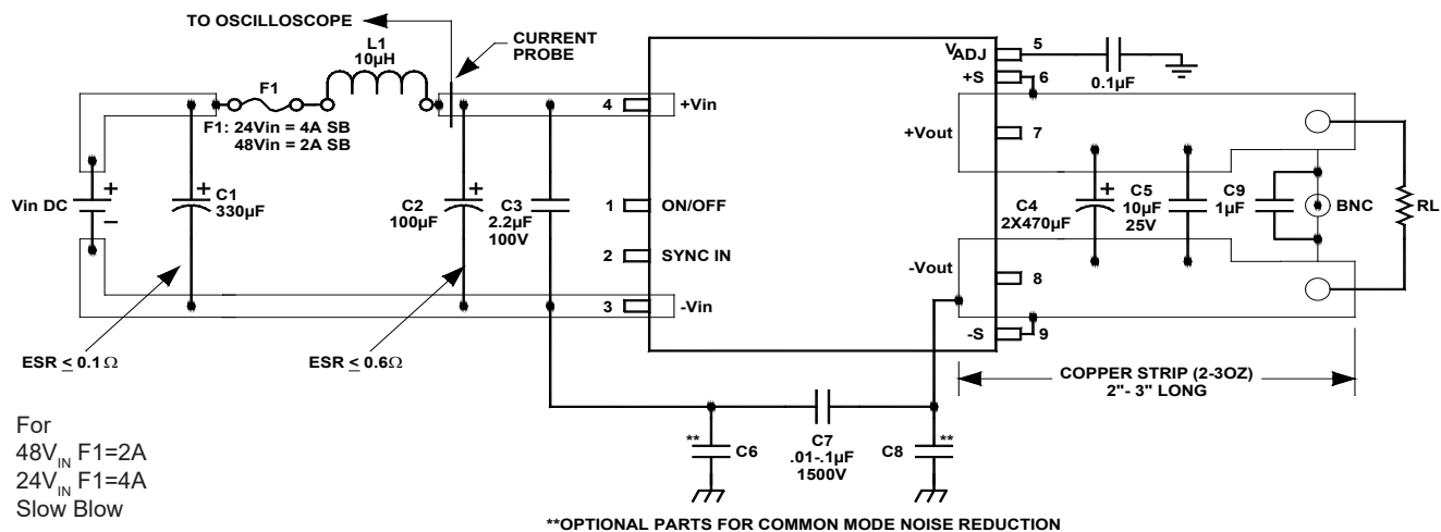
FIGURE 2A. Setup for further output ripple reduction
