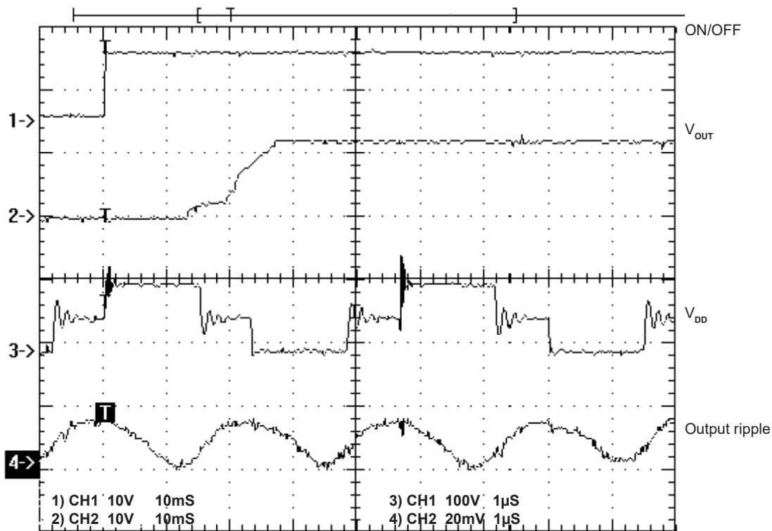
FIGURE 2B. Turn-on delay and output ripple of EB30S12/48
