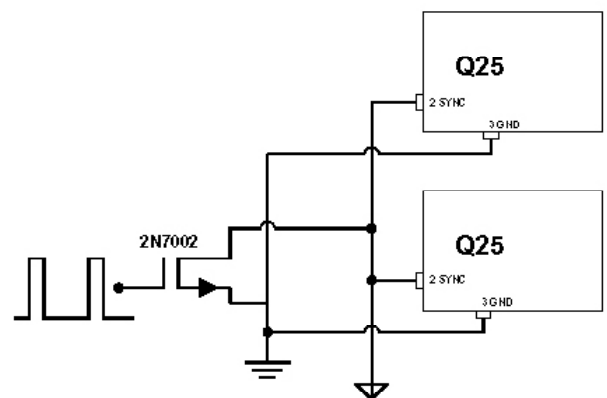
FIGURE 10. SYNC of multiple devices
