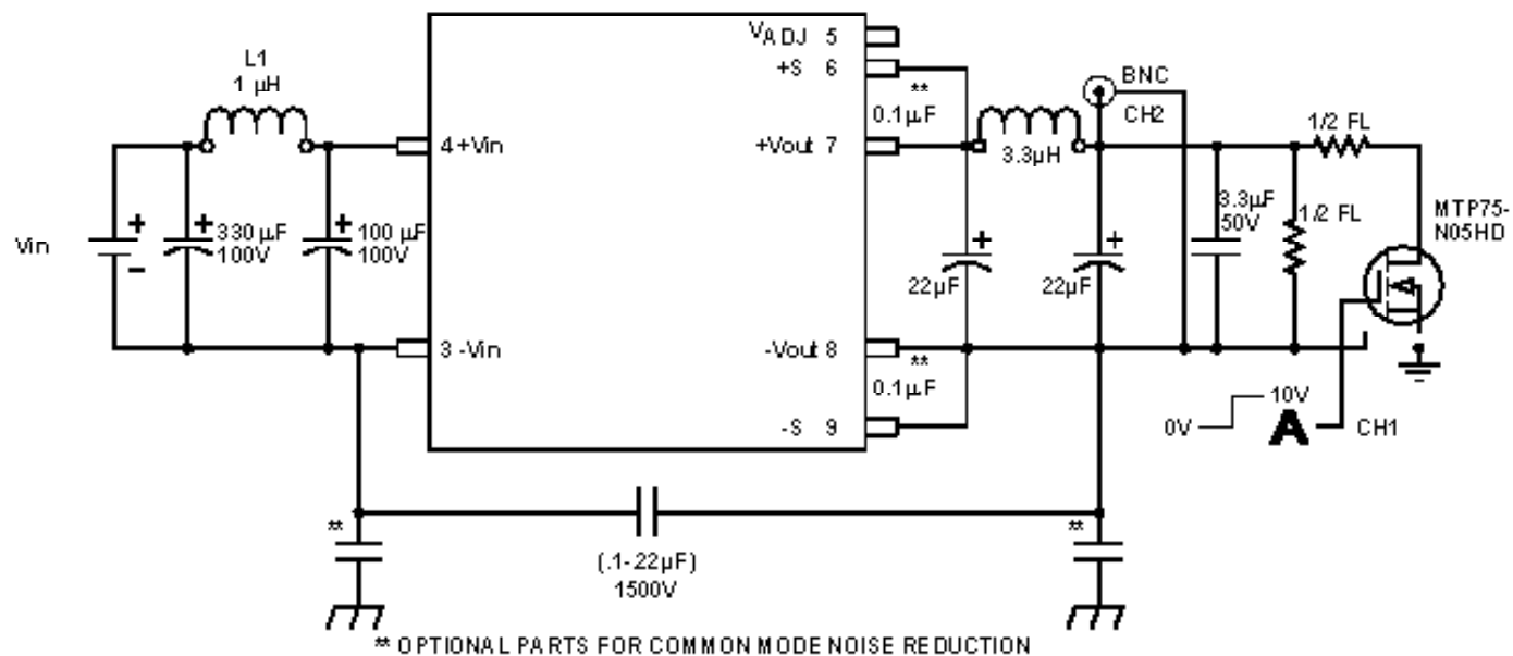
FIGURE 3. Setup for transient response measurements
