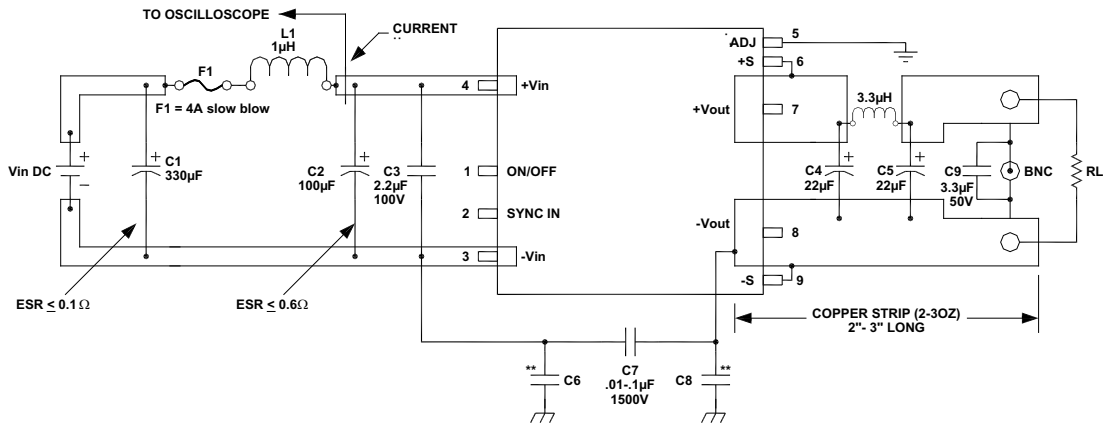
FIGURE 2. Setup for further output ripple reduction
