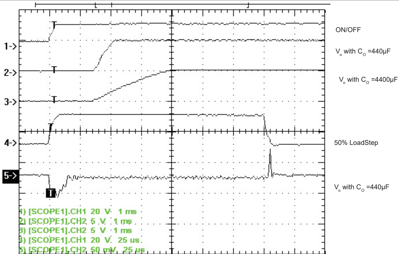
FIGURE 3. EAL50S5/24 Turn on delay with soft start and transient response
