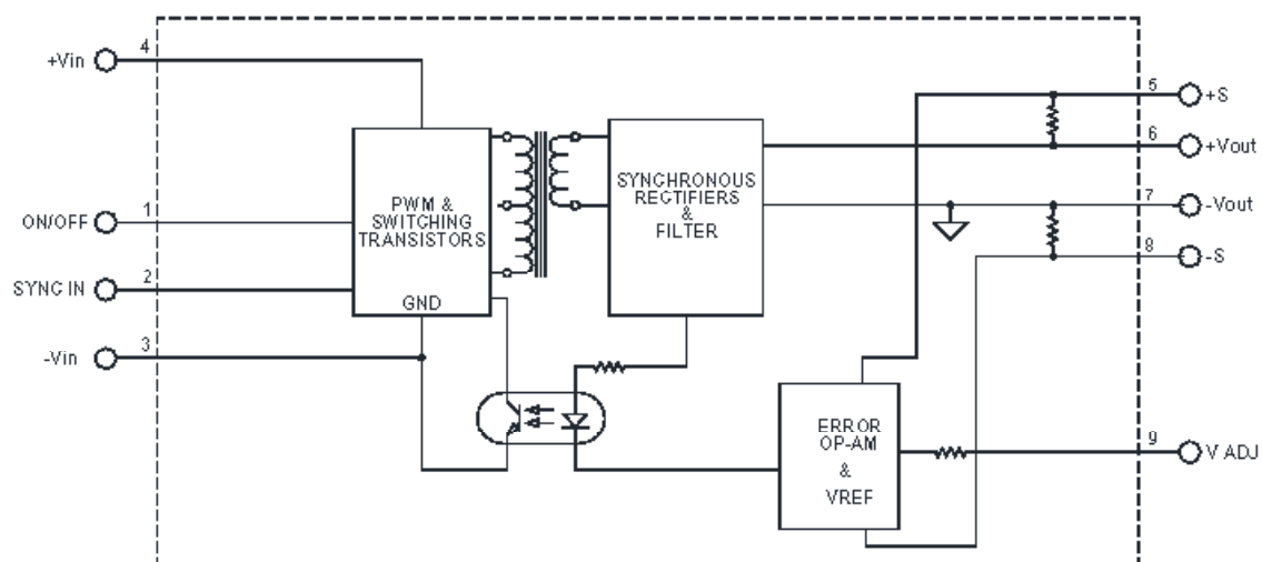
Typical Block Diagram of BHE30 Single Output Converter
