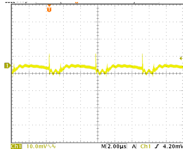
FIGURE 4. Typical output ripple of BHE30S5/6000/Q24 as shown in Figure 5 with an additional 180uF@16V low esr capacitor.
