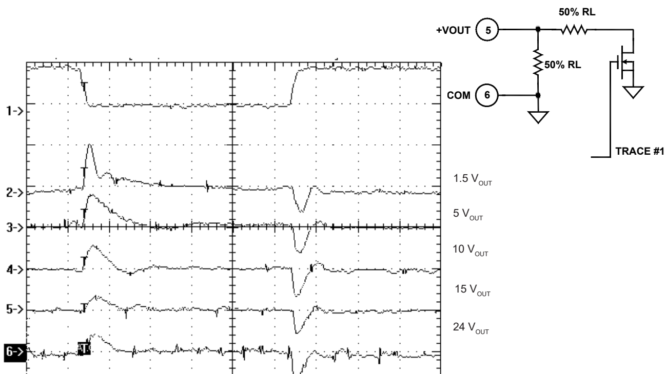
FIGURE 5. Transient Response of AD35002, I_{OUT}@1A
